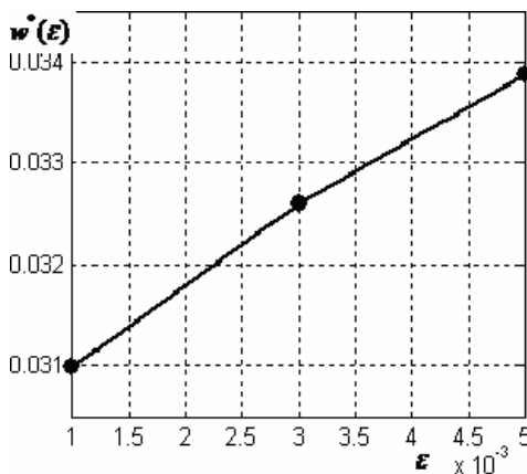
Figure 11. Numerical example: The function w^*(\varepsilon)
