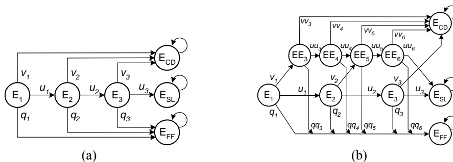
Figure 4. Ordinary two-inspection strategy state graph (a) for initial two-inspection program and switching to the double inspection frequency state graph (b).
