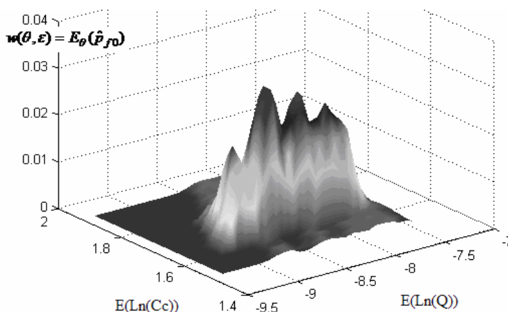
Figure 10. Function w(\theta, \varepsilon) = E_\theta(\hat{p}_{f0}) for \varepsilon = 0.001
