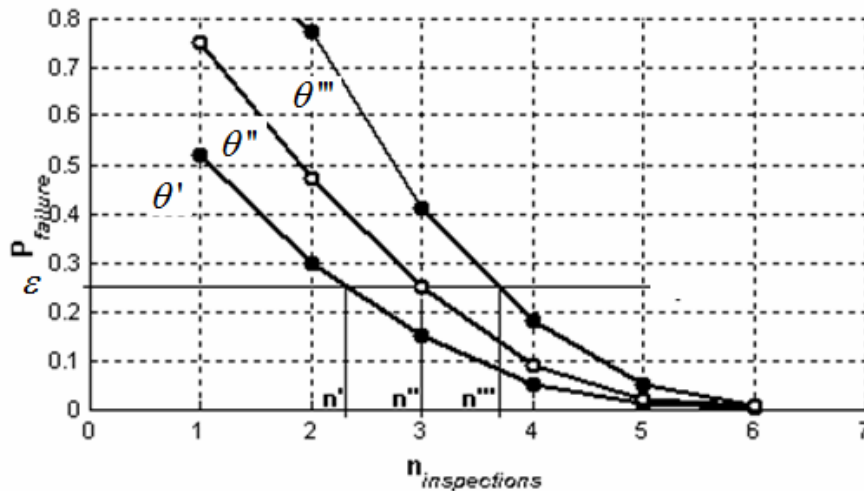
Figure 9. Choice of number of inspections as function of allowed failure probability for different parameter \theta
