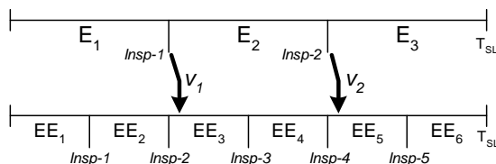
Figure 3. Switching to double inspection frequency for initial two-inspection program
