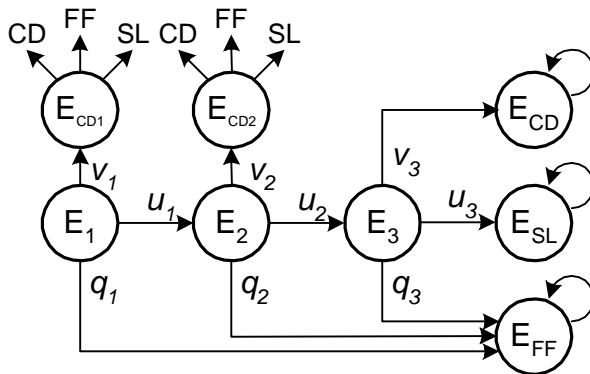
Figure 5. Switching to the double inspection frequency reduced state graph for initial two-inspection program
