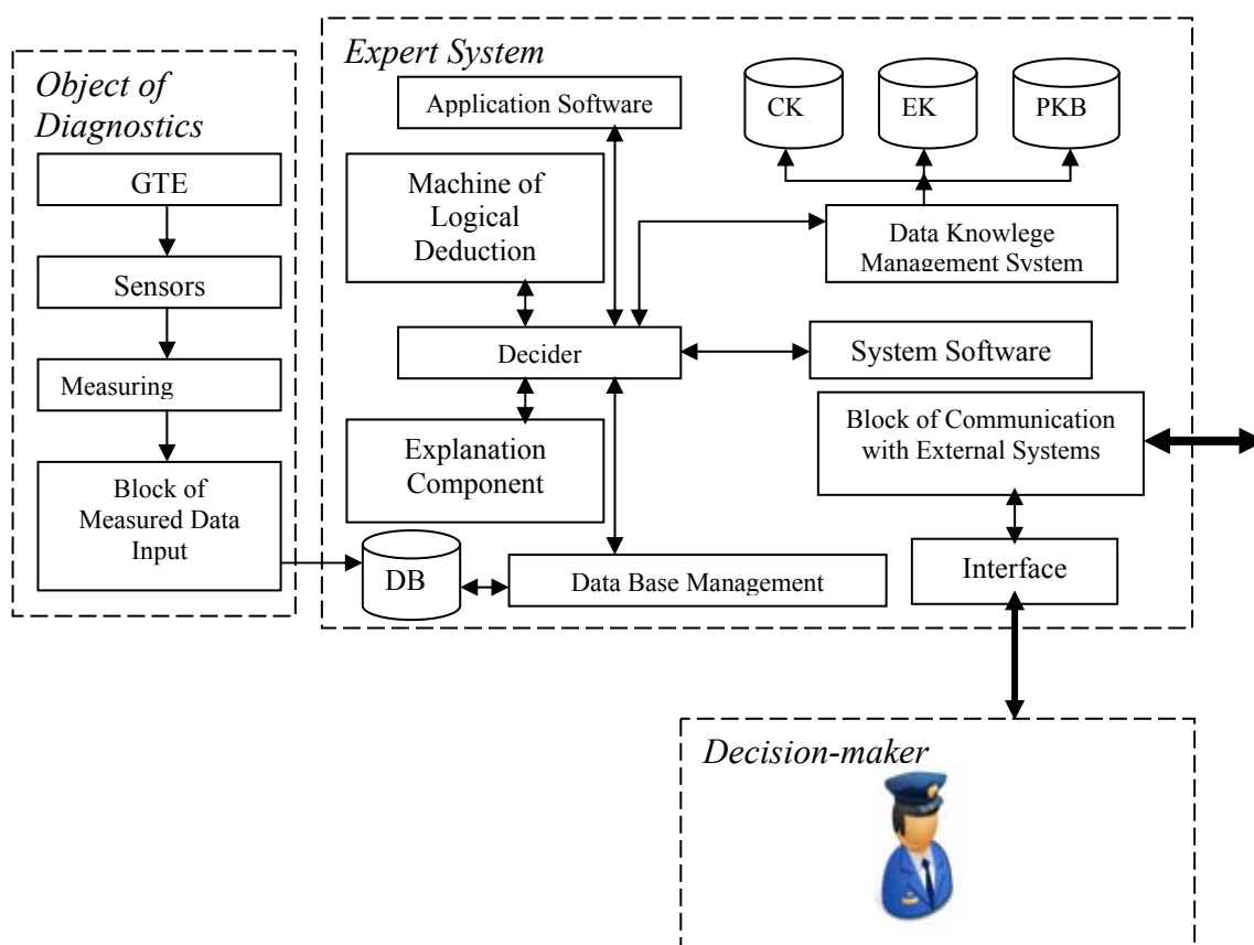
Figure 1. Structure of the expert system of monitoring the GTE status condition
