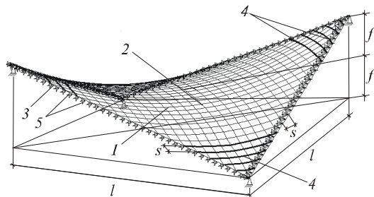
Fig 2. Calculation scheme of primary element
