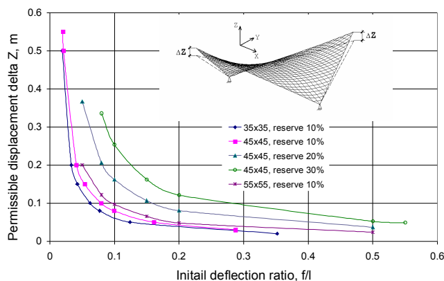
Fig 3. Permissible displacements of supports of primary element depending on initial deflection of primary element
