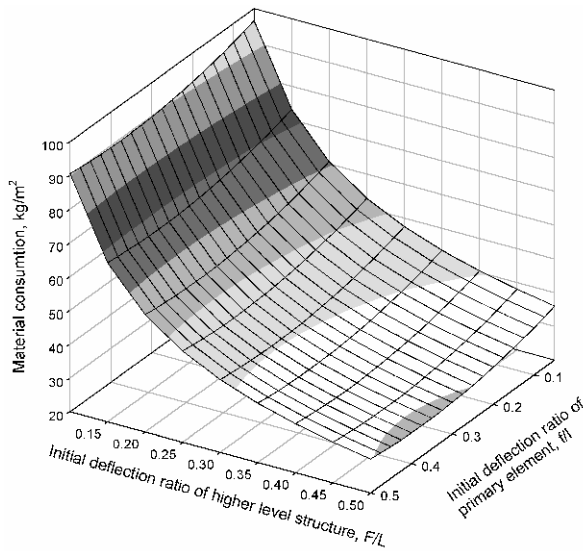
Fig 4. . Material consumption of hierarchic cable structure depending on initial deflections of primary element and higher level cable structure (primary element size 45x45m, external load 0,48 kN/m 2 ); L - span of the higher level cable structure
