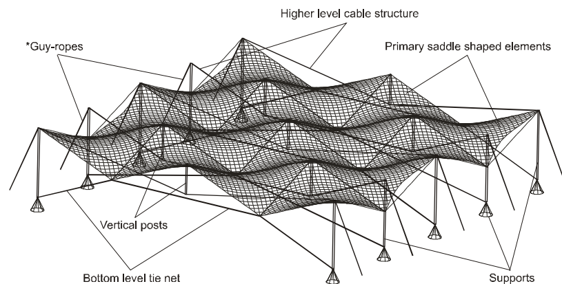
Fig.1. Simplified variant of hierarchic cable structure module
