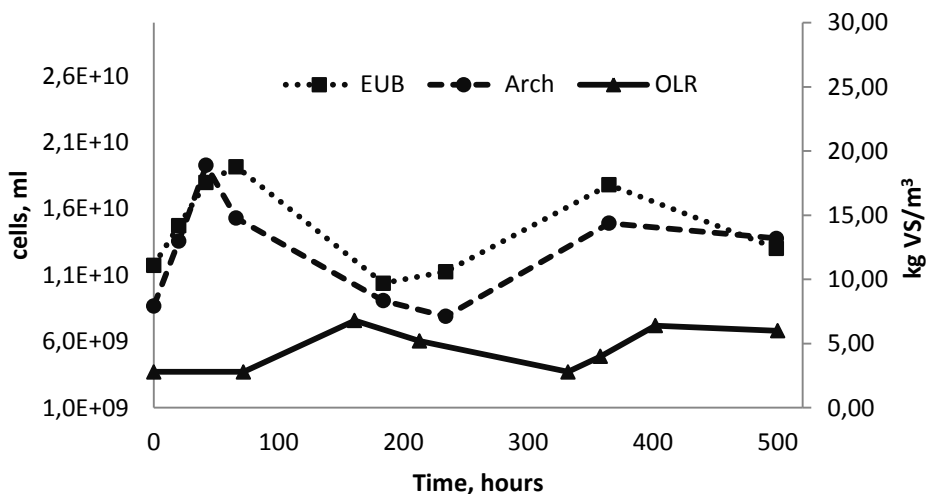
Figure 4. Amount of Archaea (Arch) and Eubacteria (EUB) in the reactor during anaerobic treatment with various ORL.
