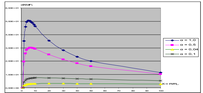
Fig. 1 Dimensionless characteristics dX/dFo = f(X) of vapor bubble growth, water, P=101.3kPa , super-heating 10K. Value of \alpha (0,04; 0,1; 0,5; 1,0) here means index of "evaporation-condensation" \alpha_{lv} for water, varying from 0,004 to 1,0 in accordance of kinetic theory.
