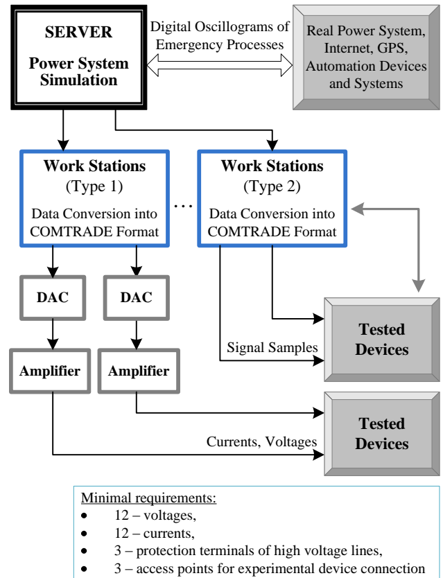
Fig. 2. Power Systems Simulator structure
