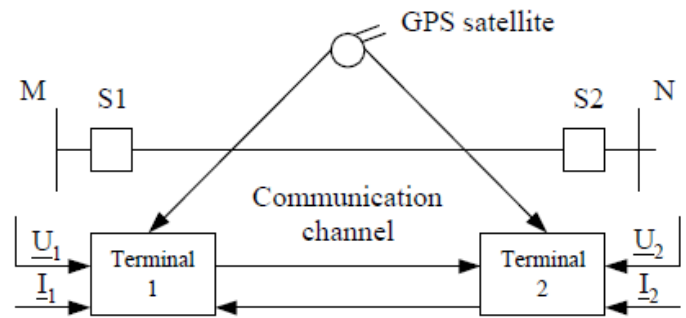
Fig. 8. Diagram of the line protection
