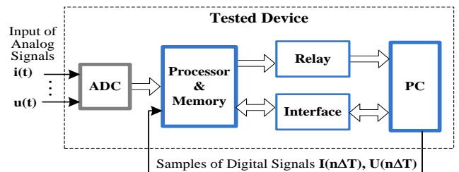
Fig. 3. Microprocessor-based automation device structure
