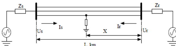
Fig. 10. Model of protected object
