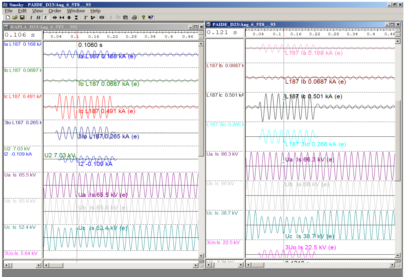
Fig. 5. Process of short-circuit in high voltage transmission line
