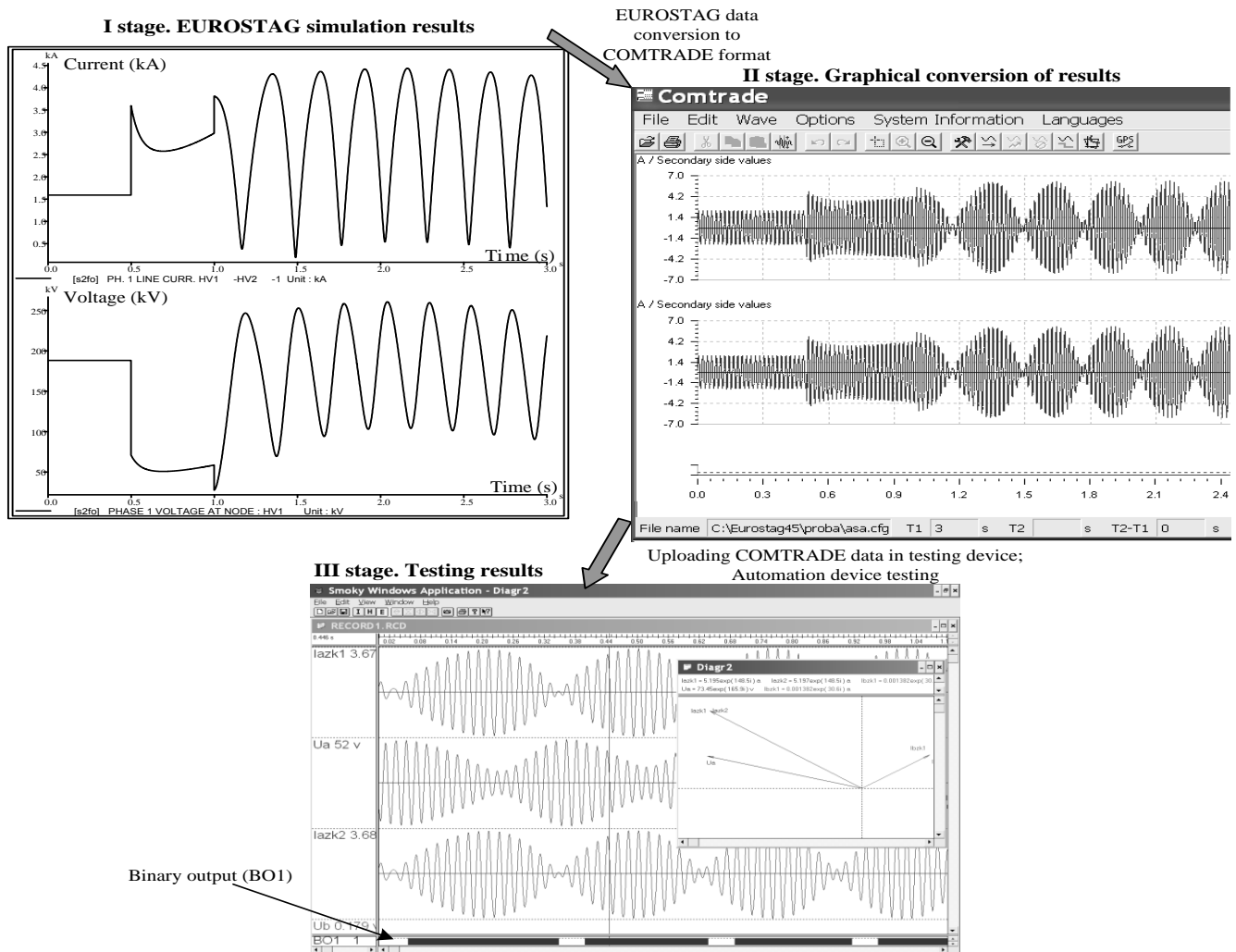
Fig. 4. Power system regime simulation and tested relay operation
