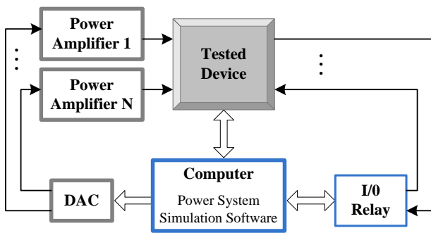
Fig. 1. Testing system configuration
