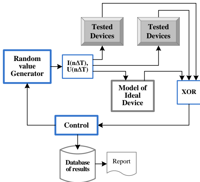
Fig. 9. Testing in the space of device signals
