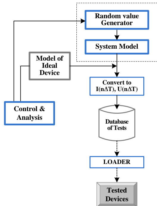
Fig. 11. Structure of system for testing in the space of protected object's parameters
