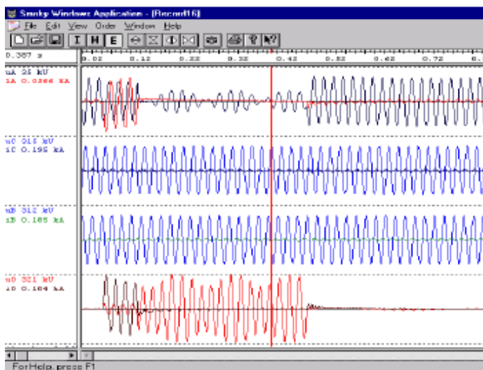
Fig. 7. Complex test example
