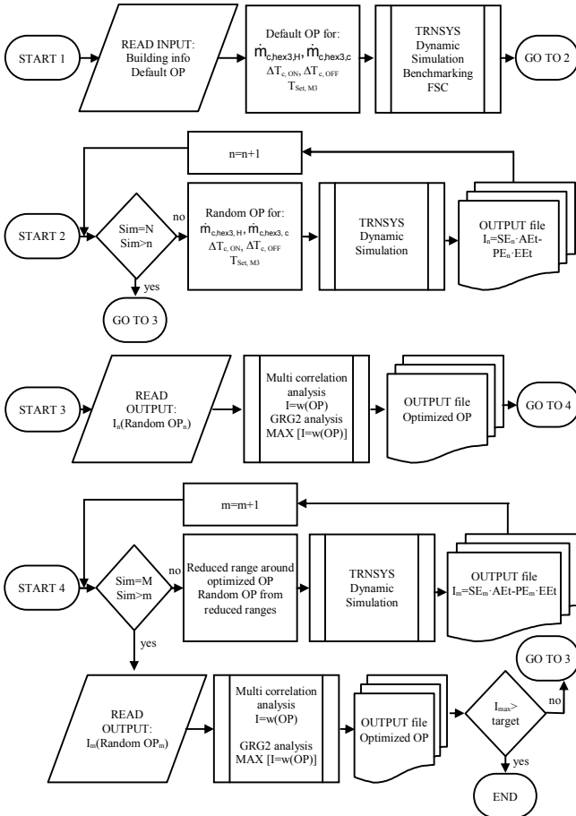
Figure 2. Algorithm used for optimisation of the solar combisystem under exam
