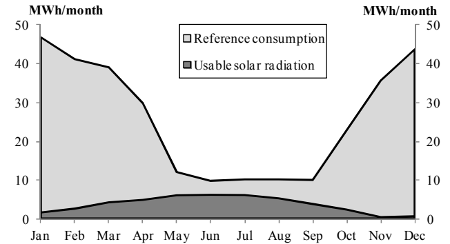
Figure 4. Results of calculations of FSC values, in MWh
