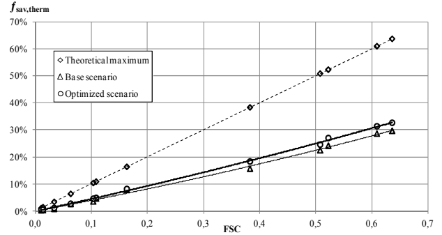
Figure 6. Comparison of the optimized solar combisystem with the upper and lower benchmark values.
