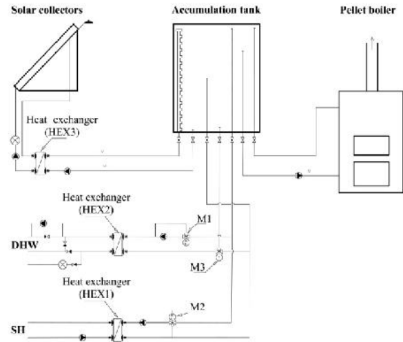
Figure 1. Simplified hydraulic scheme for the solar combisystem
