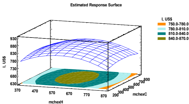
Figure 5. Variation of I depending from the flow rates at the primary and secondary side of the solar heat exchanger.
