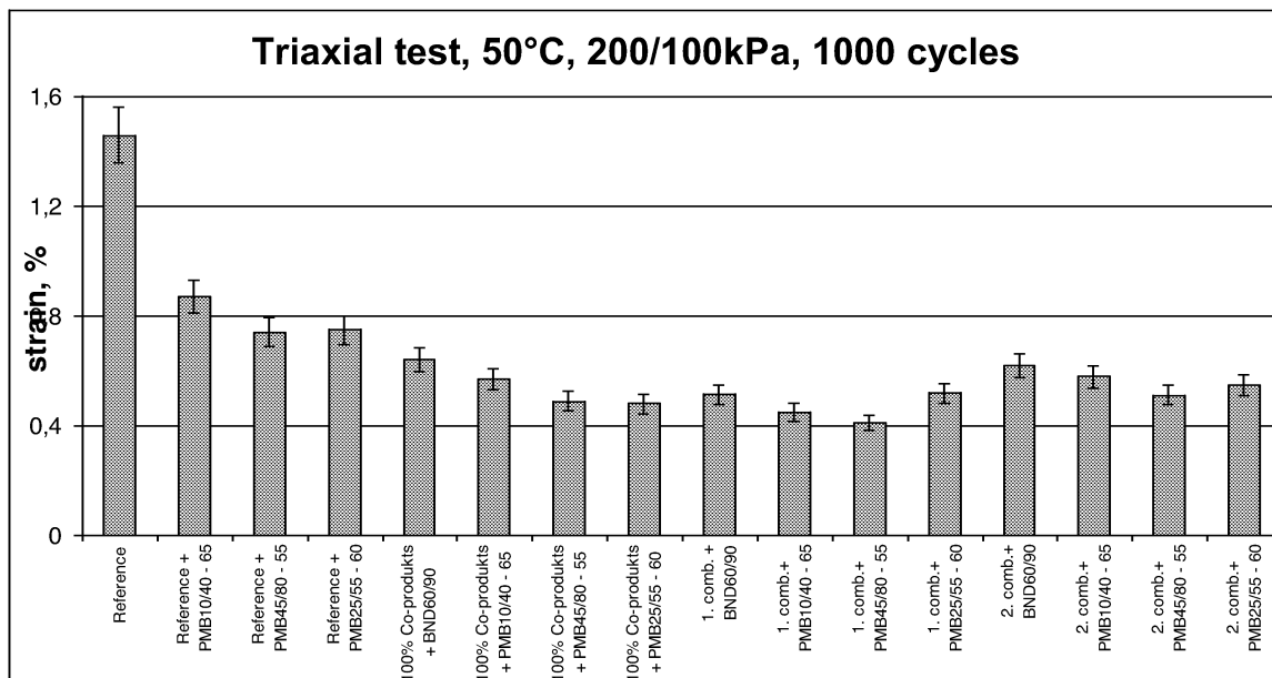
Figure 4. Triaxial test results
