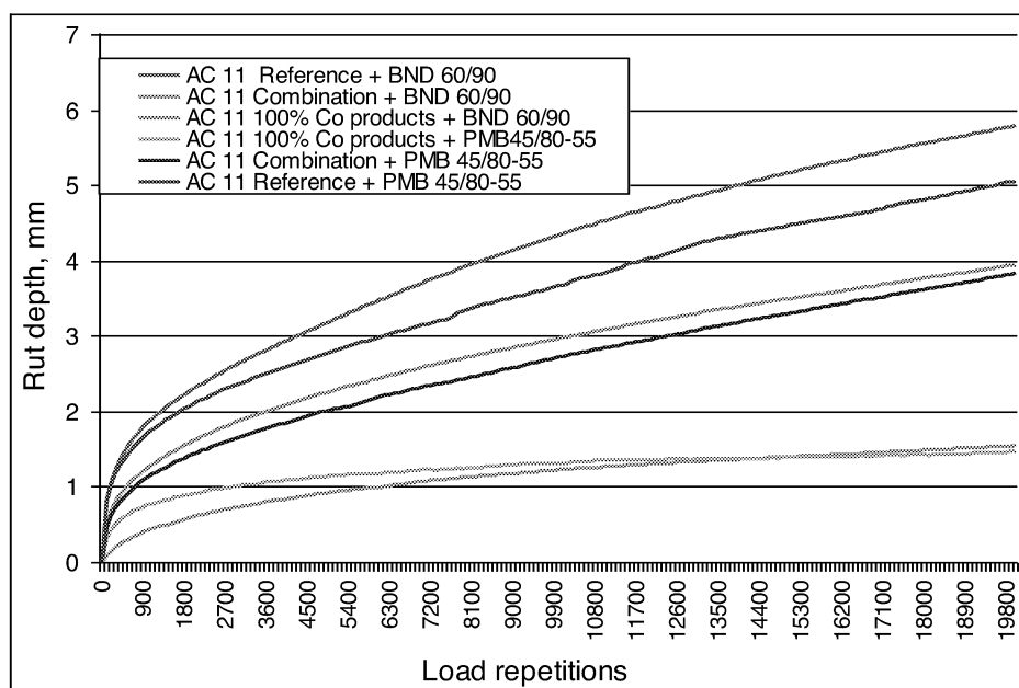
Figure 5. Wheel Tracking test
