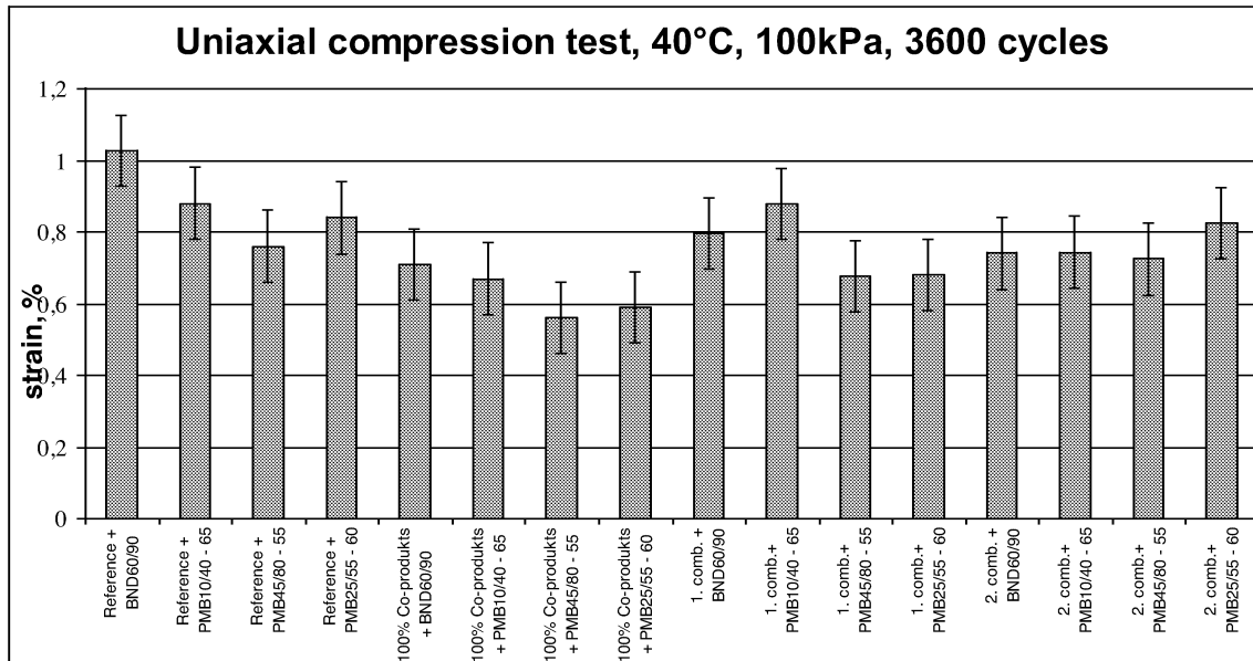
Figure 3. Uniaxial compression test results
