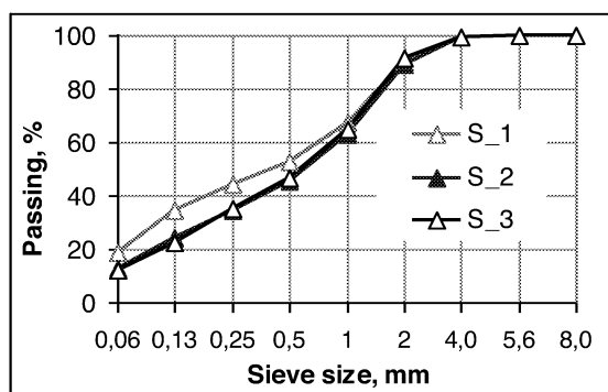
Figure 1. Particle size distribution of dolomite sand
