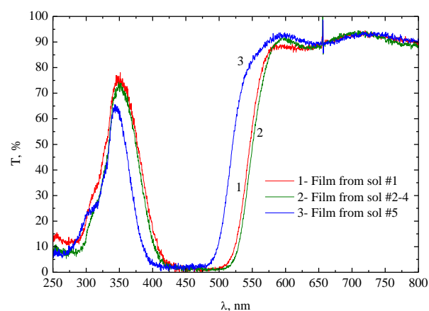
Fig. 2. Transmission spectra of samples films
