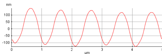
Fig. 4. The dependence of the surface relief modulation depth on exposure records for KRJ-8 modified and unmodified samples and AFM-image of typical grating (KRJ-8 + \text{CH}_3\text{COOH} 1:1). Recording laser wavelength is 405 nm, the grating period is 1 micron.
