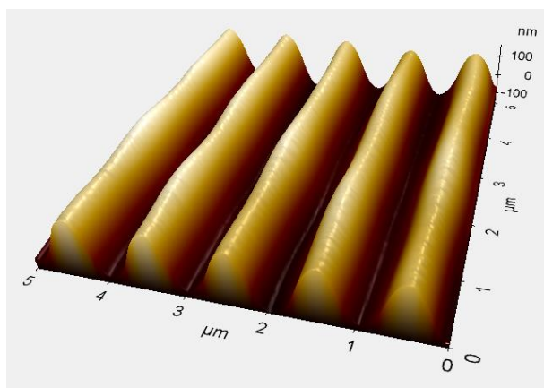
Fig. 4. The dependence of the surface relief modulation depth on exposure records for KRJ-8 modified and unmodified samples and AFM-image of typical grating (KRJ-8 + \text{CH}_3\text{COOH} 1:1). Recording laser wavelength is 405 nm, the grating period is 1 micron.
