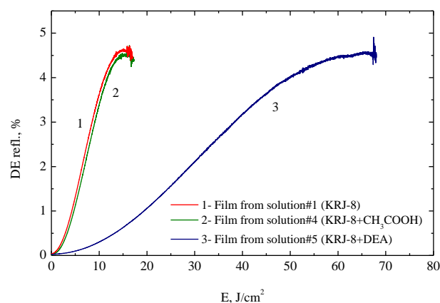
Fig. 3. The dependence of the reflection diffraction efficiency on exposure records for KRJ-8 modified and unmodified samples. Recording laser wavelength is 532 nm, beam polarization are \pm 45^\circ , intensity 0.22 \text{W}/\text{cm}^2 the grating period is 1 micron.
