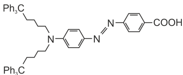
Fig. 1. Chemical structure of KRJ-8
