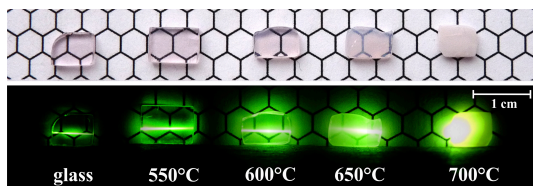
Glass and glass ceramics excited at 979 nm
